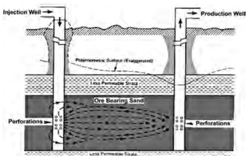
Generalized Diagram of Uranium ISL Mining Method
